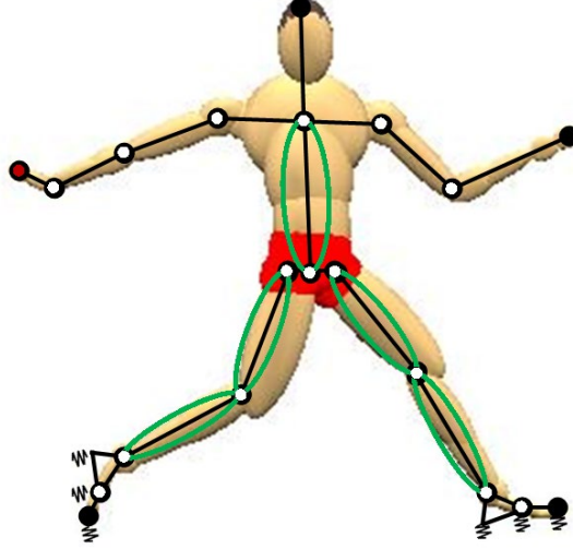
Figure 2 - 16-segment simulation model with wobbling masses within the shank, thigh and trunk segments, angle drivers at all joints (white circles) and spring-dampers at three points on each foot.
