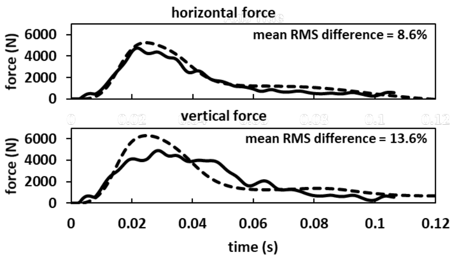
Figure 4 - Comparison of simulation (solid line) and recorded (dashed line) ground reaction forces (simulation representative of the mean RMS difference for each model variant): (a) simple planar model; (b) non-coincident hip model; (c) non-coincident hip and shoulder model.
